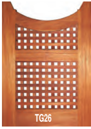
scallop full lattice gates Size Cedar Kwila 1800 x 900 x 45 $949 $1139 1300 x 900 x 45 $807 $969 1300 x 1400 x 45 $1111 $1334
