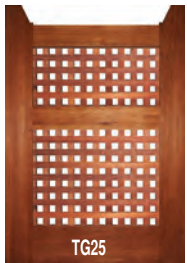
full lattice gates Size Cedar Kwila 1800 x 900 x 45 $911 $1094 1300 x 900 x 45 $758 $910* 1300 x 1400 x 45 $1041 $1250
